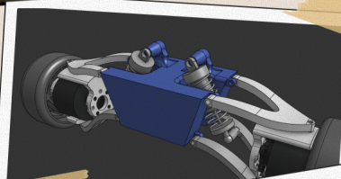
Suspension
